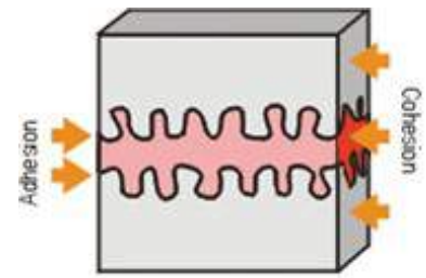
Figure 1: The types of forces in an adhesive joint. Good adhesion and cohesion are required to achieve high performance joints. Adhesives and bonding agents typically have a flow phase when they are applied, building up adhesion, followed by a hardening phase during which the cohesive strength builds up.
