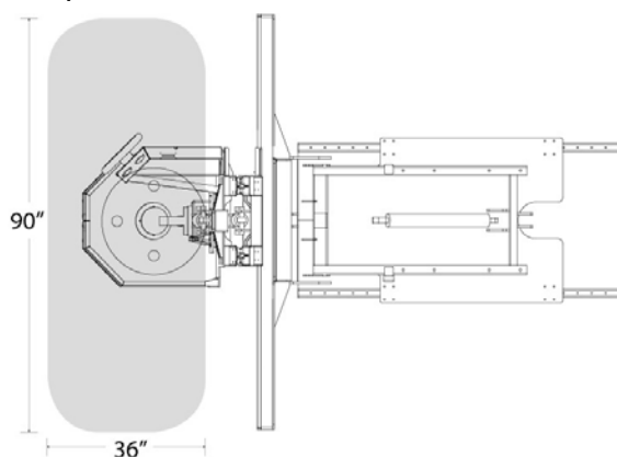
Fully manoeuvrable Traversacor™ core-zone extension system
